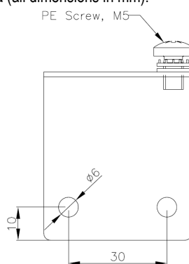
Fig 1. Fixing holes for the Xbeam™ XL EX Antenna (all dimensions in mm).
