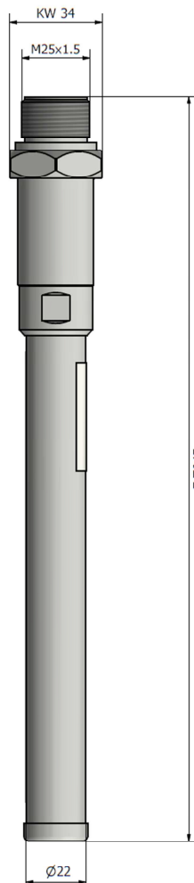
Fig 2. Physical dimensions of the Xbeam™ XL EX Antenna (approx. dimensions in mm).
